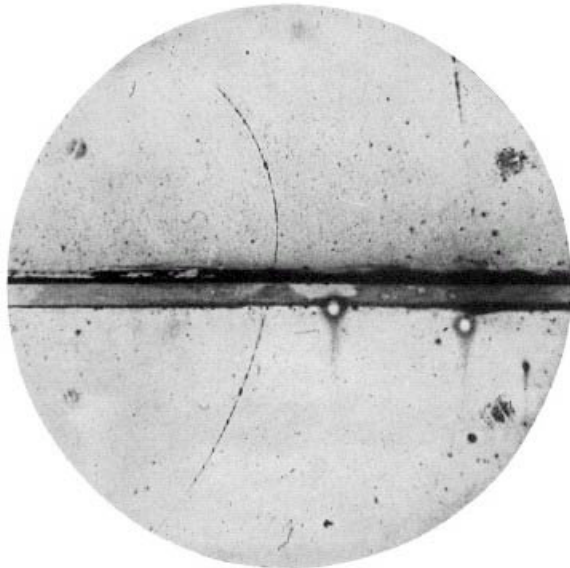
FIG. 1. A 63 million volt positron ( H_D=2.1 \times 10^6 gauss-cm) passing through a 6 mm lead plate and emerging as a 23 million volt positron ( H_D=7.5 \times 10^4 gauss-cm). The length of this latter path is at least ten times greater than the possible length of a proton path of this curvature.
